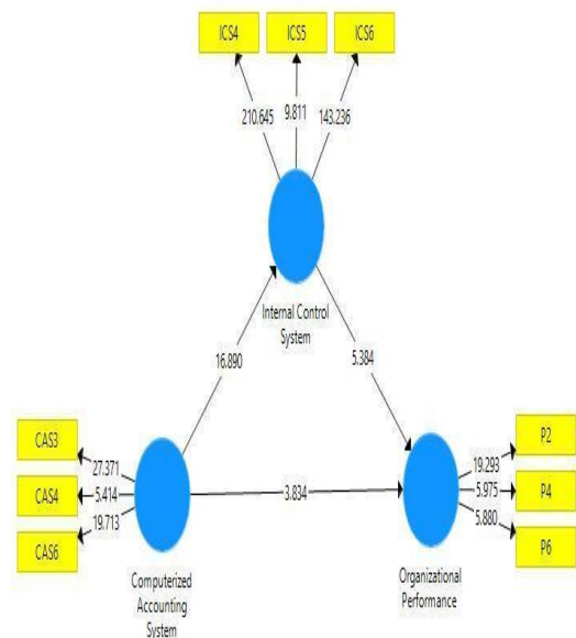
Figure 3. Structural Model
