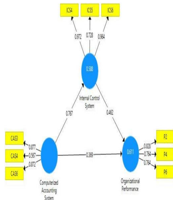
Figure 2. Measurement Model
